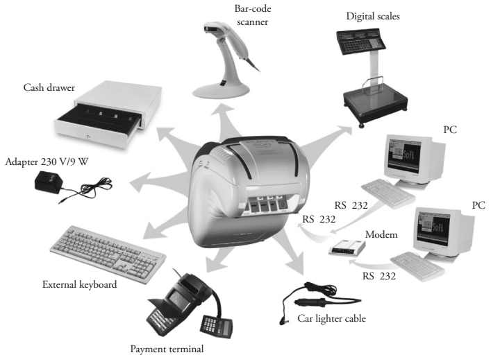
Figure 2.2 > External devices connectible to Euro-500T/TX Handy ECRs.
