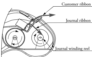
< Figure 2.7 Inserting paper tapes into ECR printer (side view).
